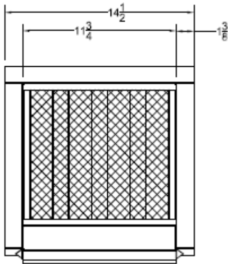
Back View
